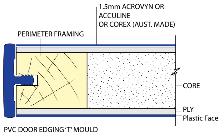
Full faced plastic protected door.
